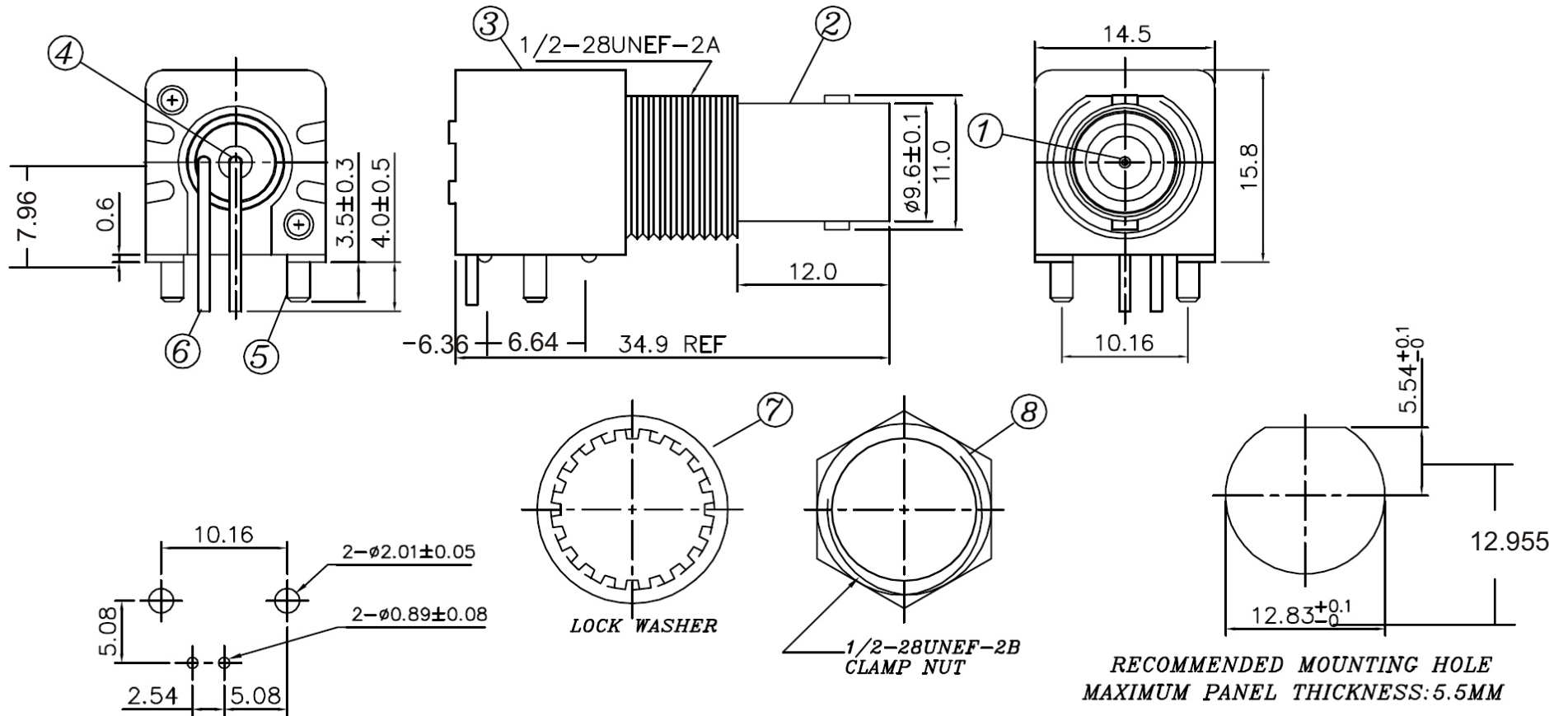
RECOMMENDED PC BOARD LAYOUT WITHOUT MOUNTING POSTS
