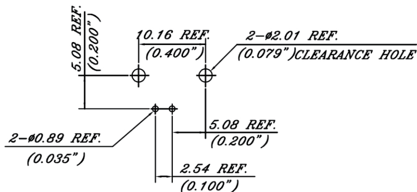
PCB HOLE CONFIGURATION
