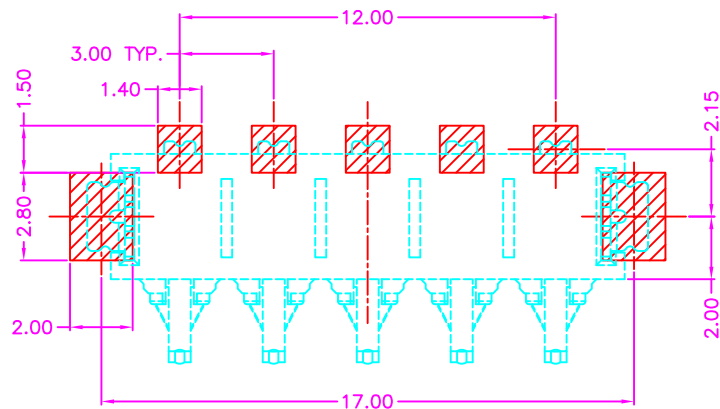
P.C.B. LAYOUT TOP VIEW \pm 0.05
