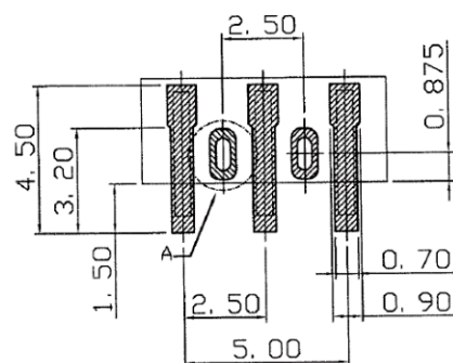
RECOMMENDED PCB LAYOUT TOLERANCE±0.05mm
