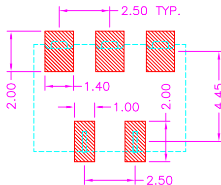
P.C.B. LAYOUT TOP VIEW \pm 0.05
