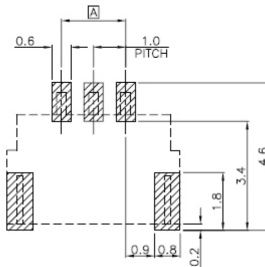
PCB LAYOUT
