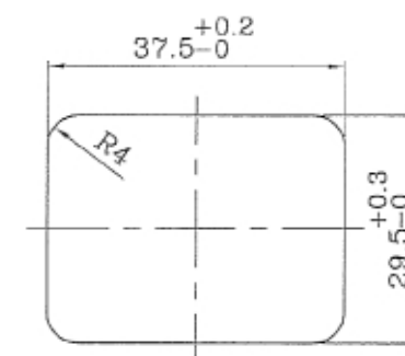
PANEL CUT-OUT
