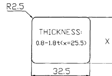
PANEL CUT-OUT
