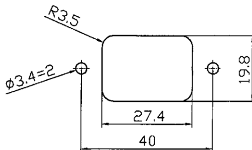
PANEL CUT-OUT
