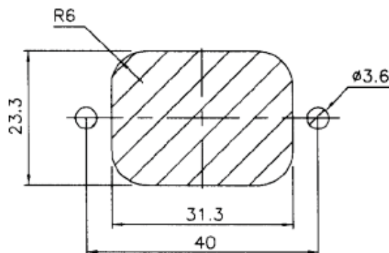
Panel Cut-Out
