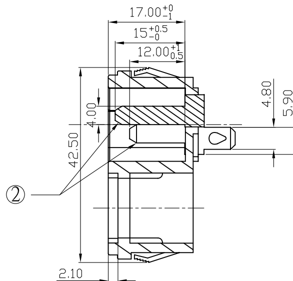
SECTION: A-A
