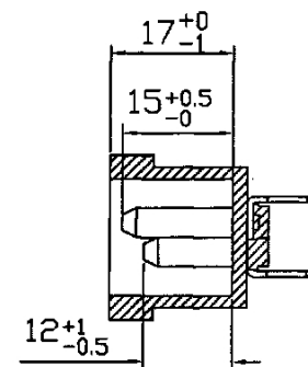
SECTION. AL
