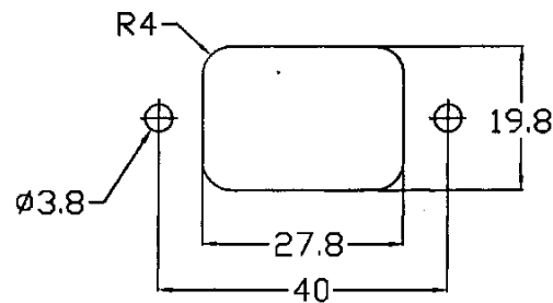
PANEL CUT-OUT
