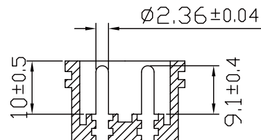
SECTION A-L
