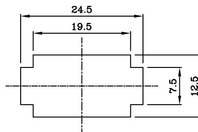
PANEL CUT-OUT
