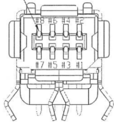
B TYPE
