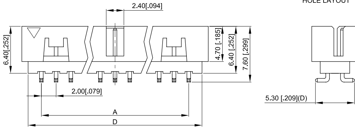
RECOMMEND P.C.B. LAYOUT HOLE LAYOUT
