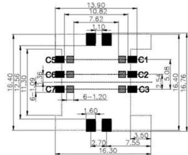
The recommended pcb layout (Tolerance=±0.1mm)
