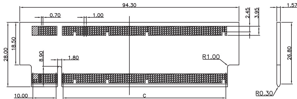
RECOMMENDED MODULE LAYOUT
