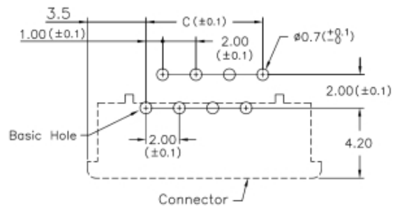
FPC/FFC INSERT DIRECTION
