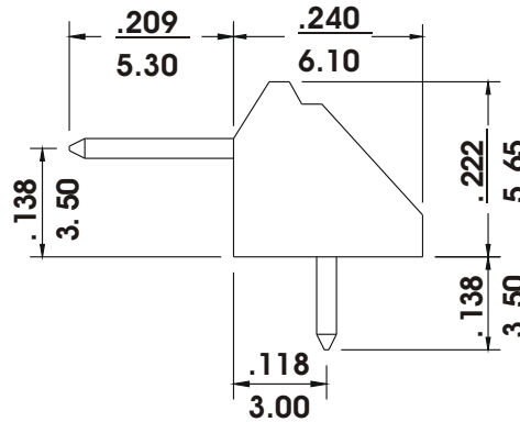
Dimensional information - inch/mm
