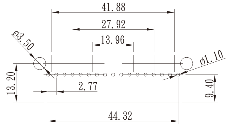
PCB LAYOUT
