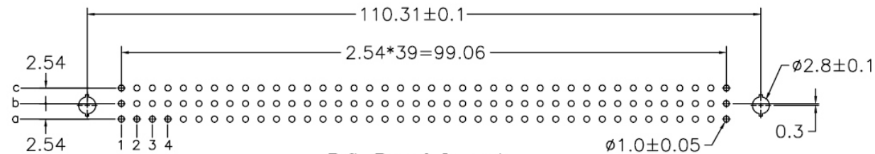
P.C. Board Layout
