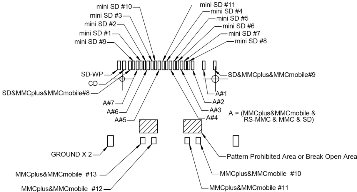
PCB LAYOUT
