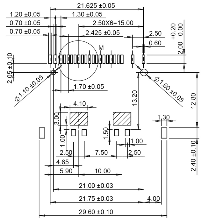
PCB LAYOUT
