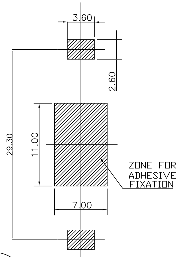
PCB LAYOUT
