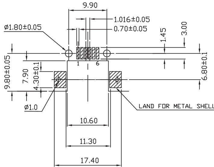
PCB LAYOUT
