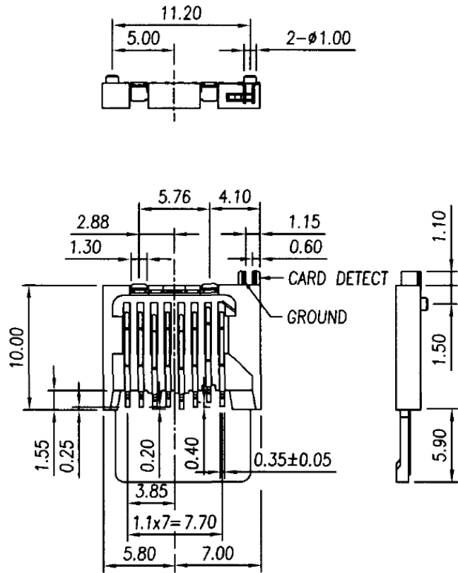
P.C.B Layout ( Top View )
