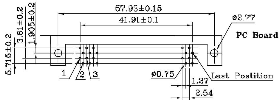
PC Board Mounting Dimensions
