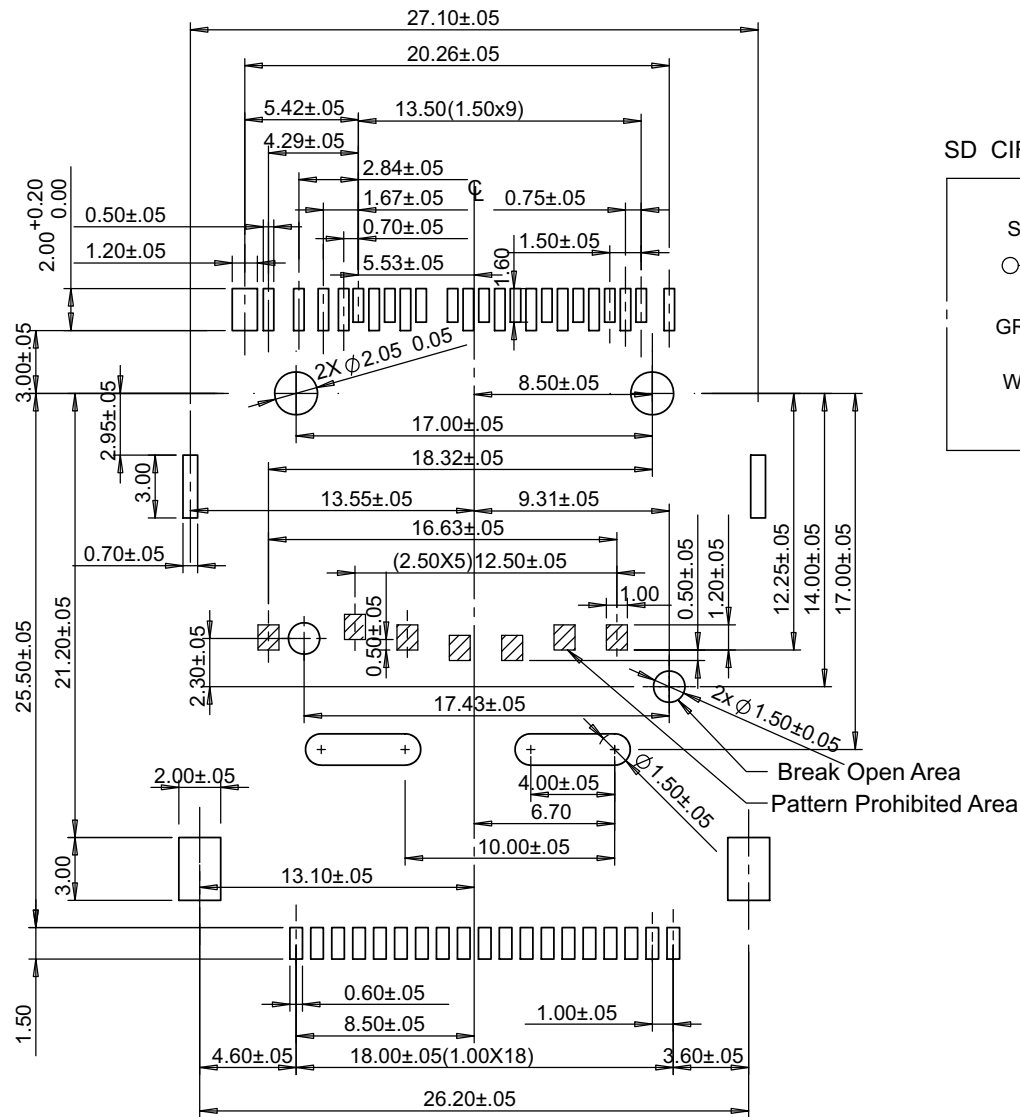
PCB LAYOUT
