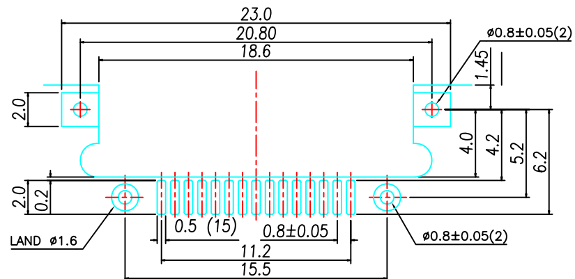
P.C.B LAYOUT TOP VIEW TOLERANCES: ±0.1
