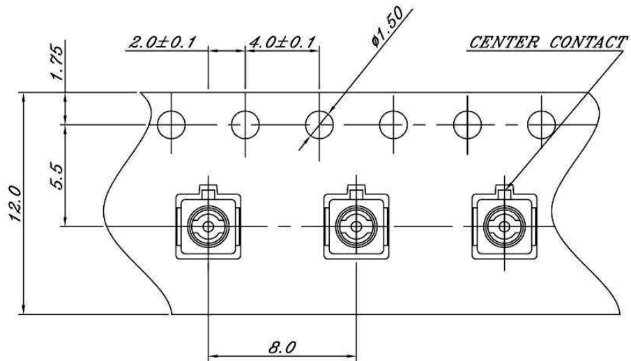
DIMENSIONS OF TAPING
