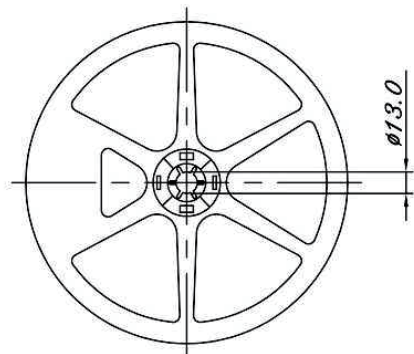
DIMENSIONS OF REEL (2500 PIECES/REEL)
