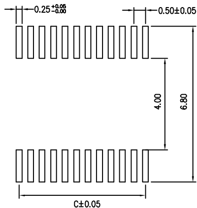
Reconnended P.C.Board Hole Layout
