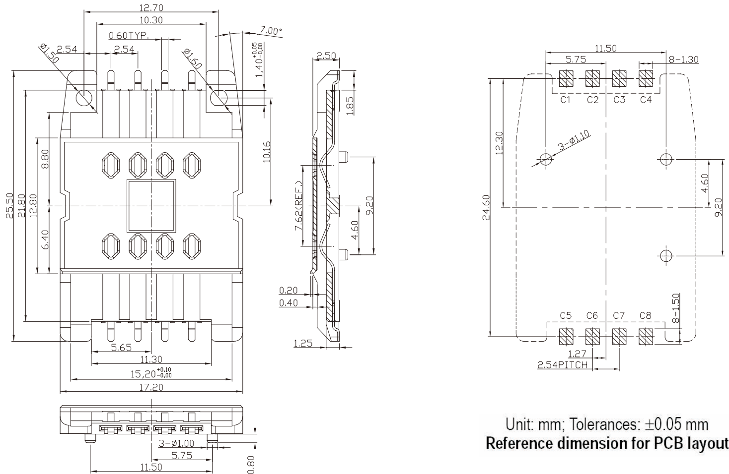
Unit: mm; Tolerances: ±0.15 mm Mechanical outline dimension
