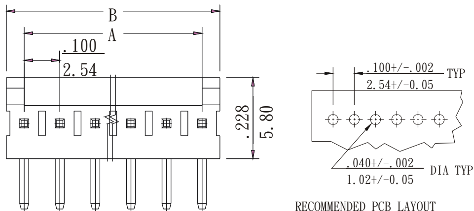
Dimensional information-inch/mm
