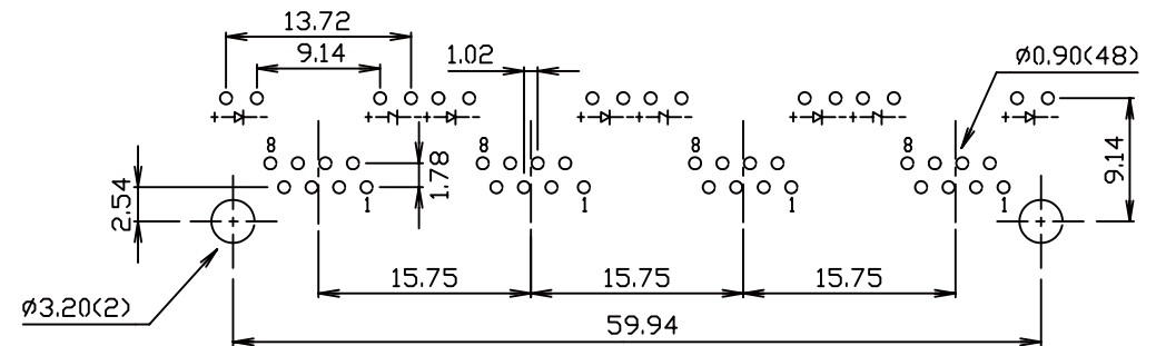
PCB LAYOUT Ref.
