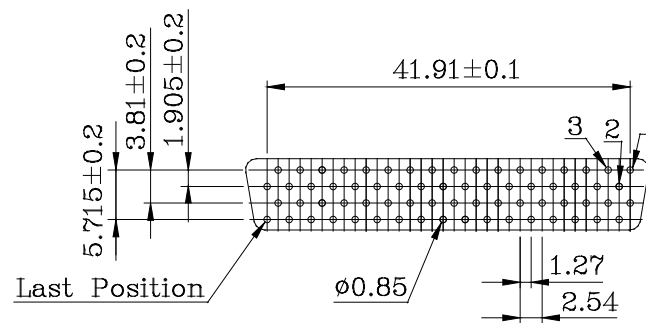
PCB Layout (B)
