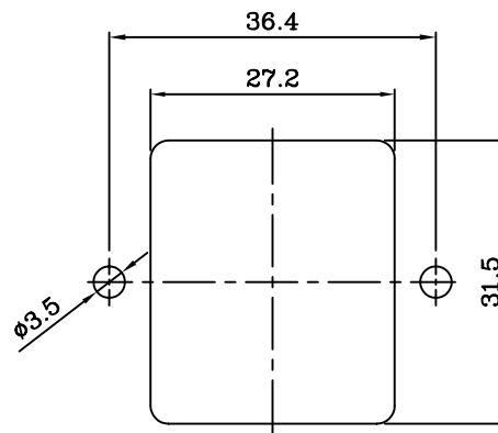
PANEL CUT-OUT
