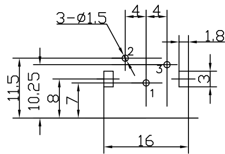
PCB HOLES(TOP VIEWED)
