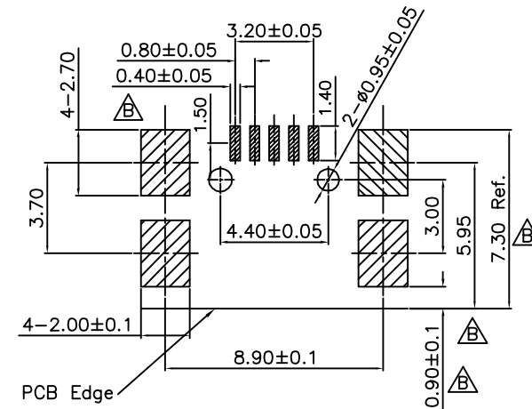
Recommended P.C.B. Pattern Layout
