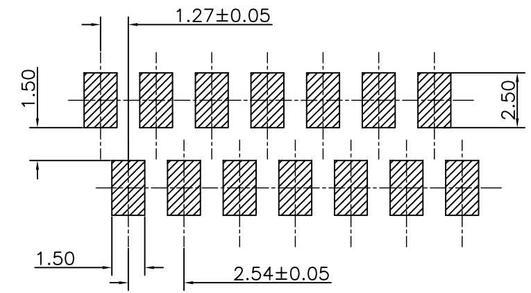
PCB Layout
