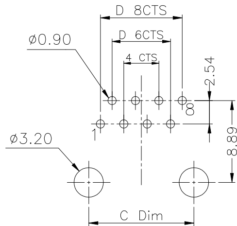
PC Board Layout PCB t=1.60mm
