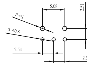
TOSLINK-LAYOUT
