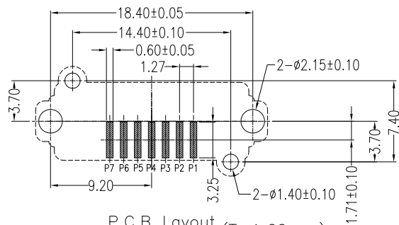
P.C.B Layout (T=1.60mm) Top View
