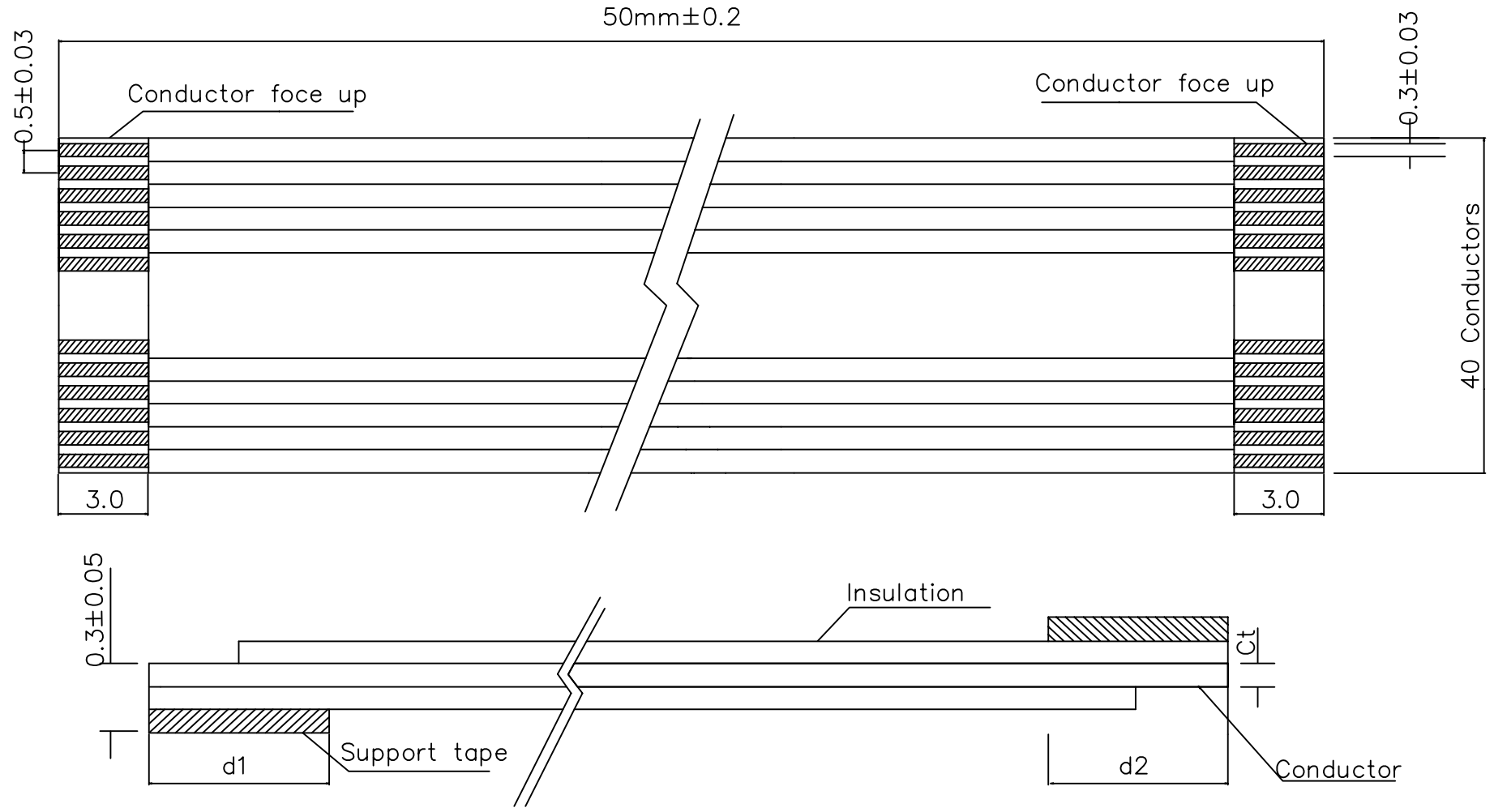
FFC 40 WAY FLAT FLEXIBLE CABLE
