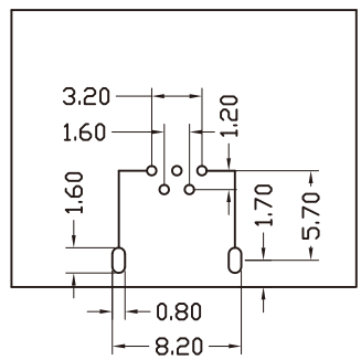
P.C.B. LAYOUT SCALE 2.00
