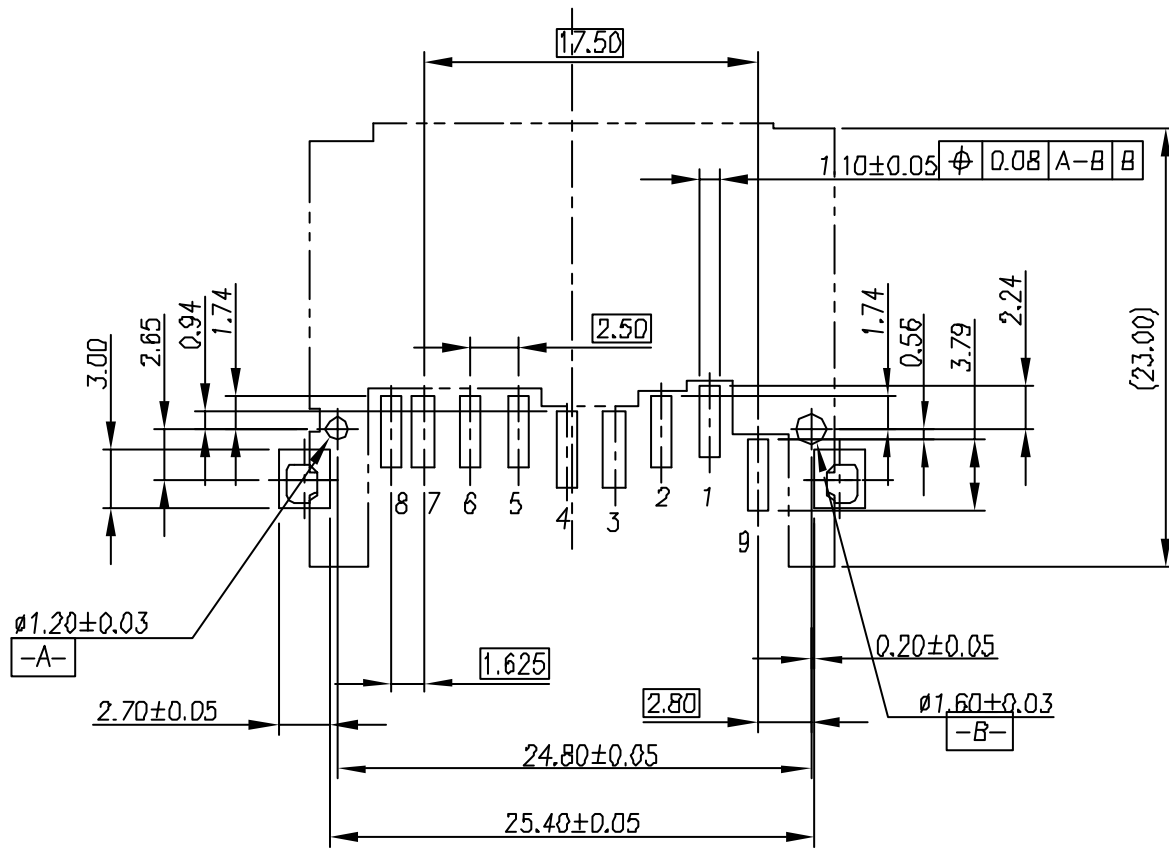
PC BOARD LAYOUT COMPONENT SIDE
