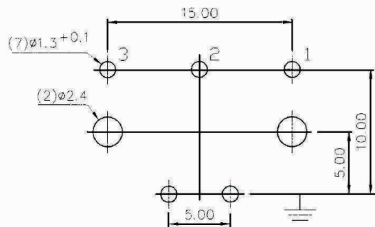
MOUNTING HOLE (TOP VIEW)
