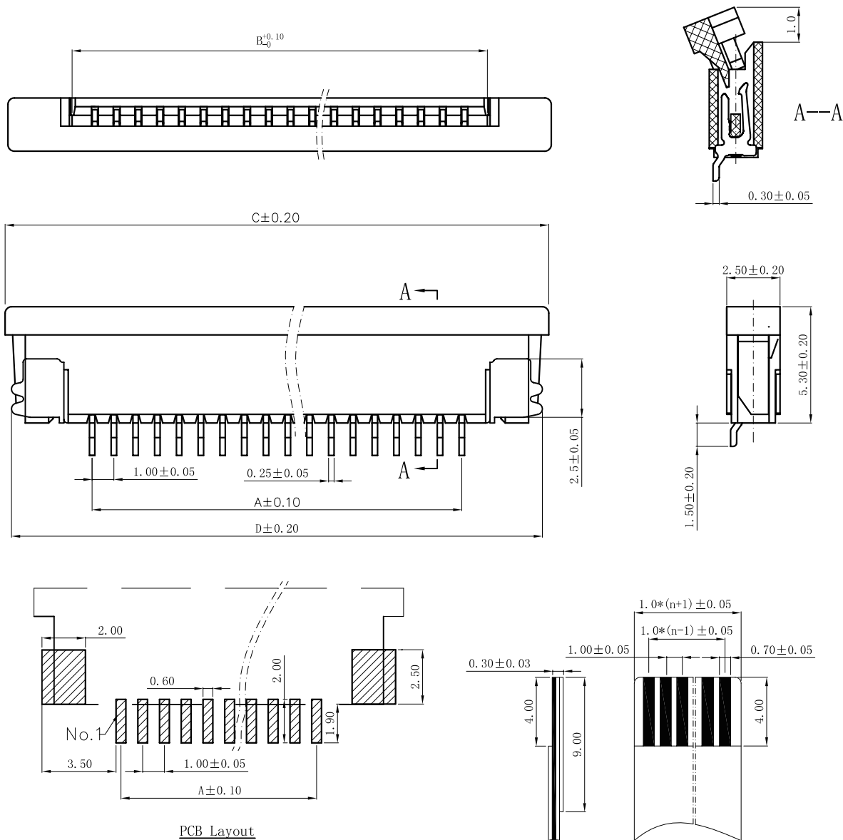
PCB Layout
