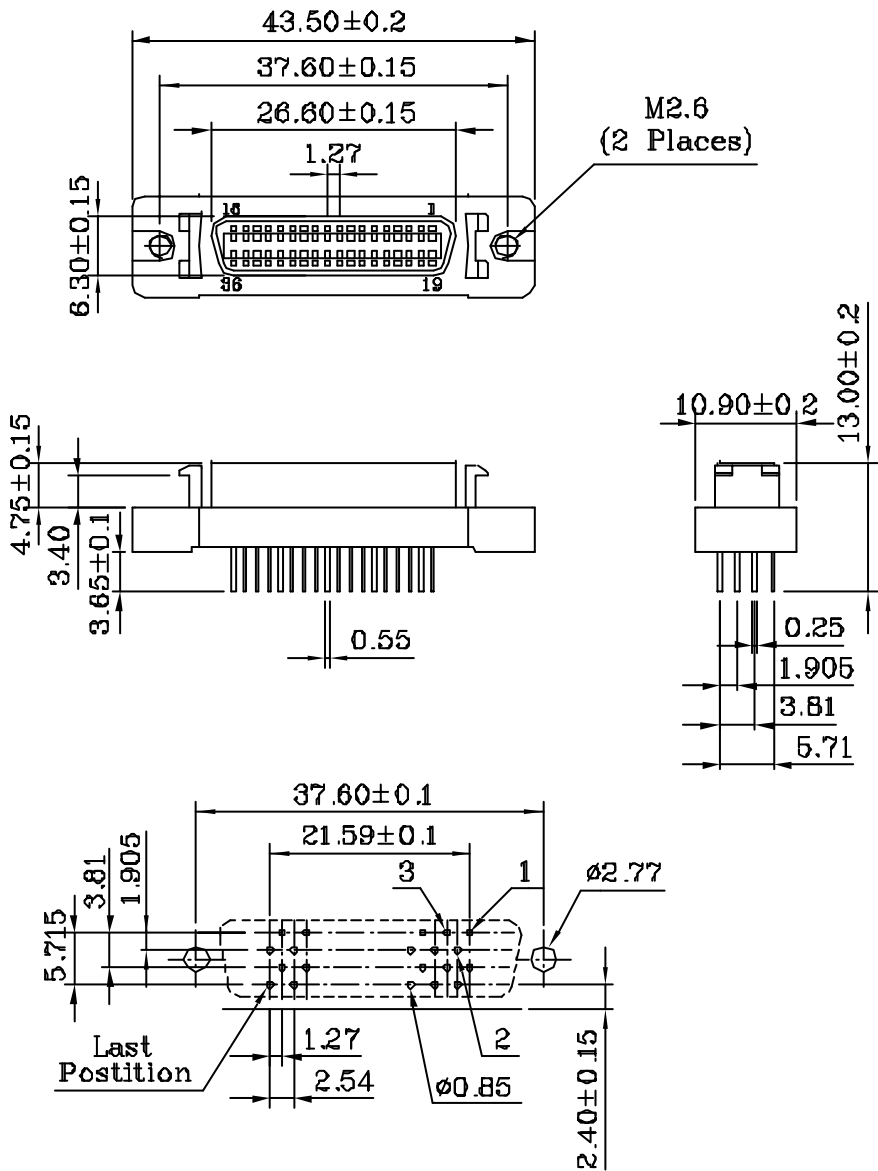
PC Board Mounting Dimensions
