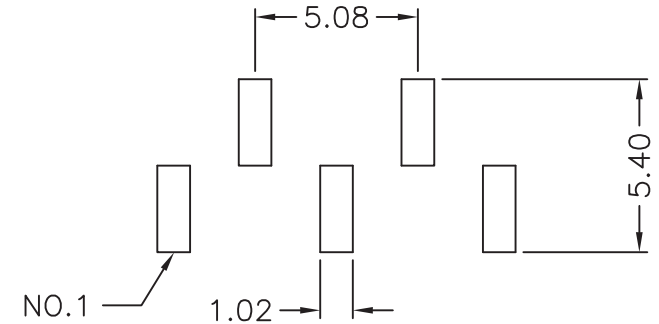
2.54 FEMALE HEADER SINGLE ROW SMT TYPE BASE 7.10H
