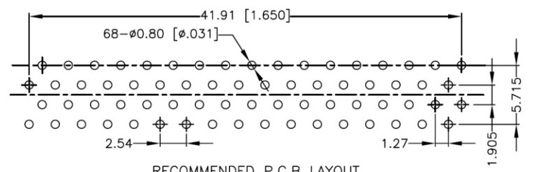
RECOMMENDED P.C.B. LAYOUT TOLERANCE ±0.05 TOP VIEW
